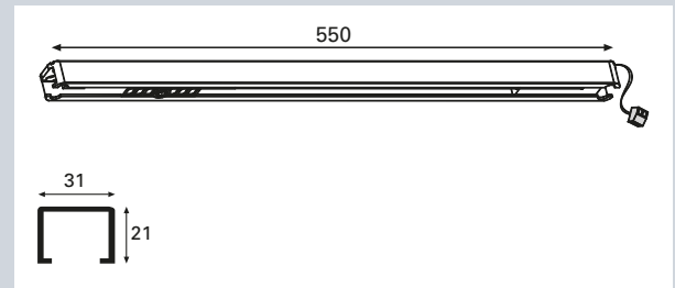
Installation slide rail ECO IS EF
