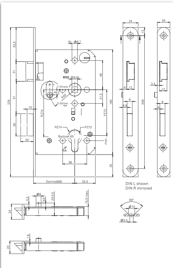
Dimensions: ECO 190
